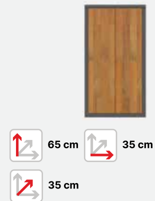
BDB.30104-A Wooden Cube Trash Can
