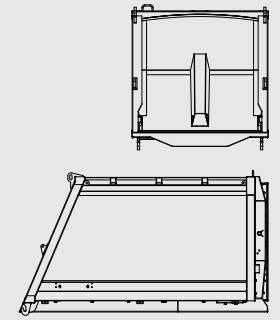
BDB.60216-A 16 M 3 Garbage Truck Body
