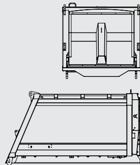
BDB.60209-A 9 M 3 Garbage Truck Body
