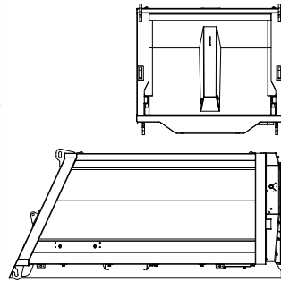
BDB.60208-A 8 M 3 Garbage Truck Body
