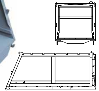
BDB.60222-A 22 M 3 Garbage Truck Body
